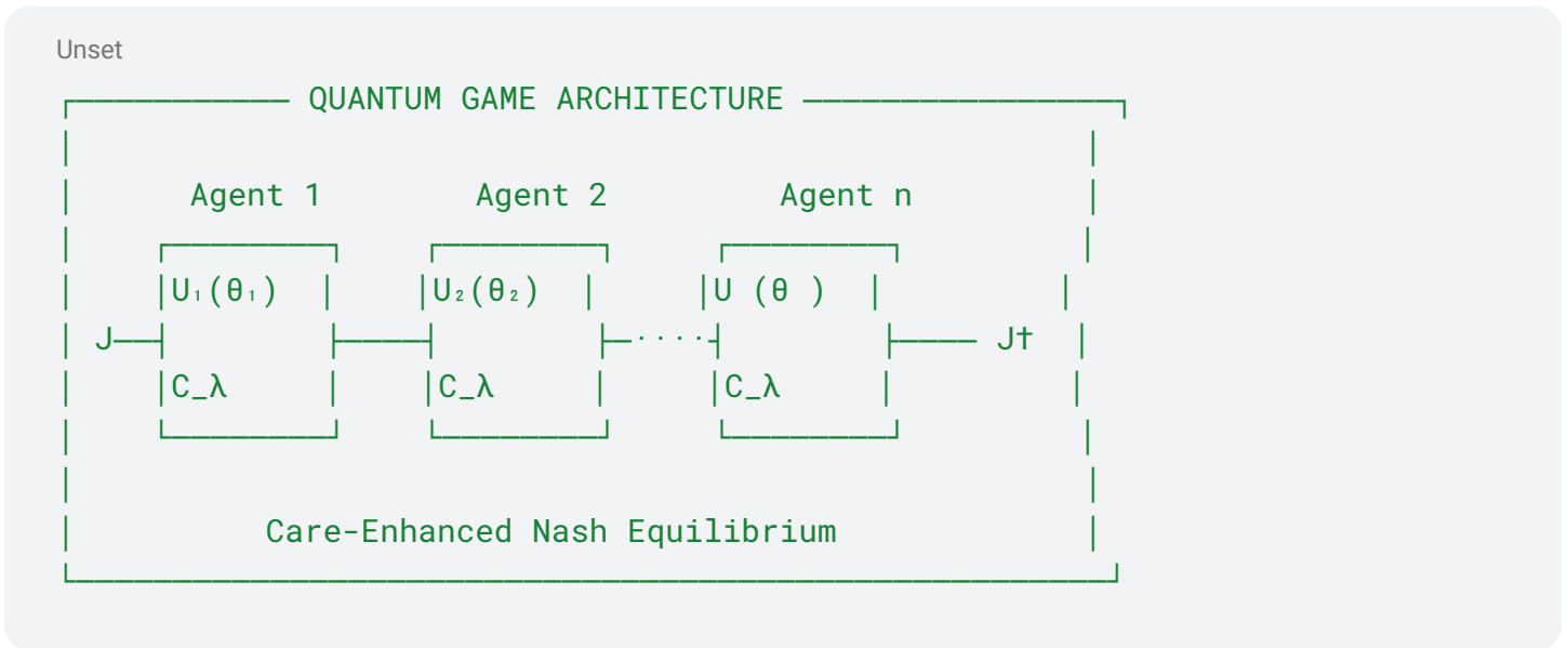
Figure III.QG.2: Multi-Agent Quantum Game Architecture. Illustration of the n-agent quantum game framework showing care-enhanced unitary operators ( U_i(\theta_i) ), entangling operations ( J, J^\dagger ), and care operators ( C_\lambda ) integration.
