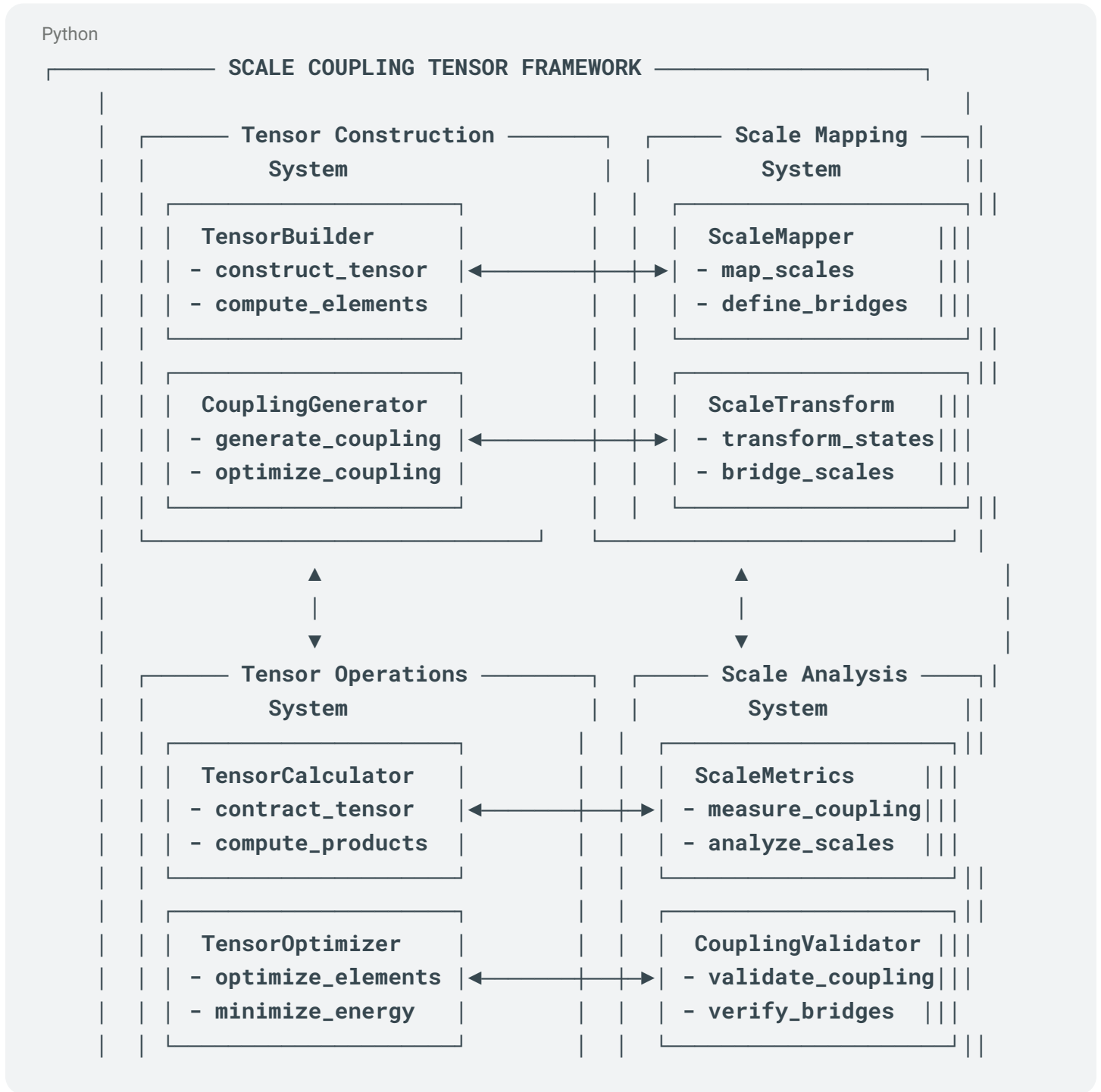
Diagram IV.M.1: Scale Coupling Tensor Framework
