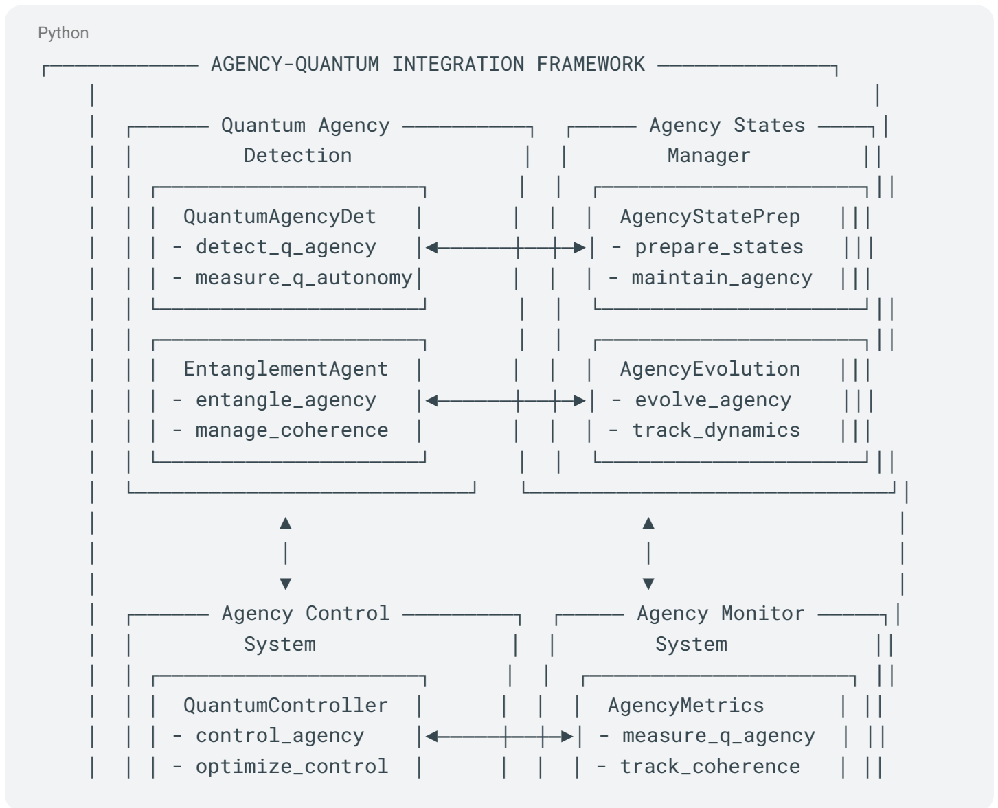
Diagram IV.J.2: Agency-Quantum Integration
