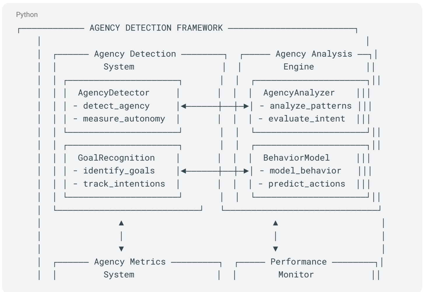
Diagram IV.J.1: Agency Framework
