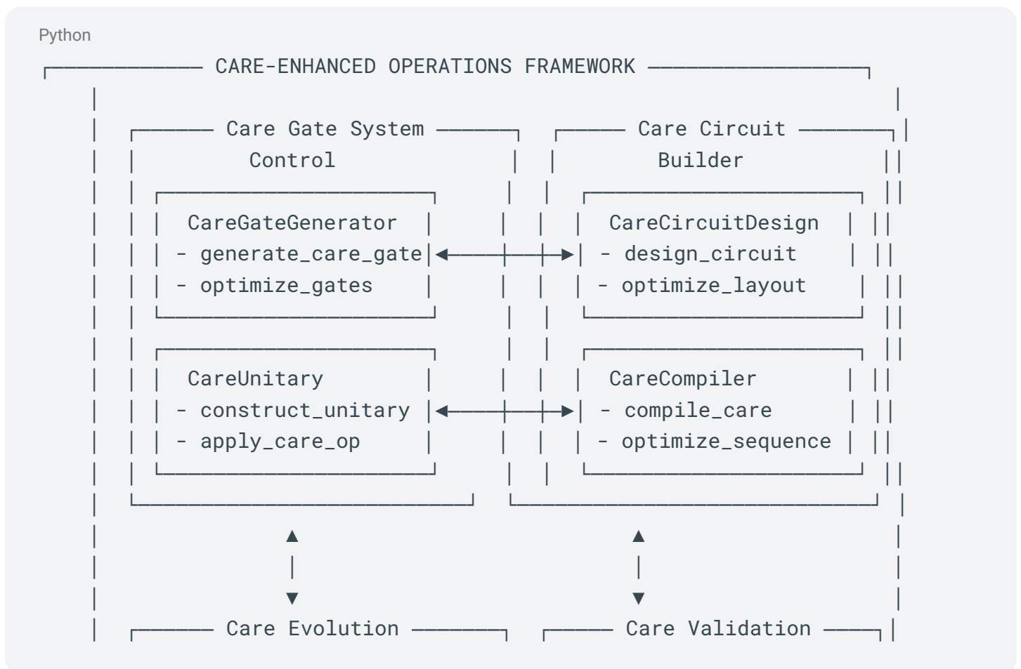
Diagram IV.G.2: Care-Enhanced Operations Framework for implementing care-enhanced quantum operations
